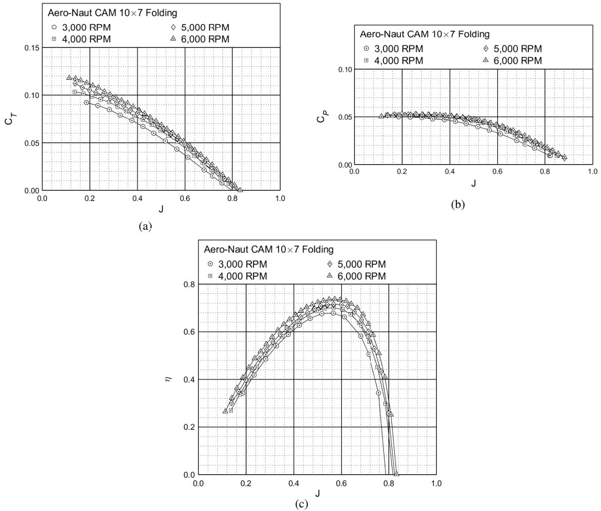
Figure 19: Performance of the Aero-Naut CAM 10×7 folding propeller: (a) thrust coefficient, (b) power coefficient, (c) efficiency.
