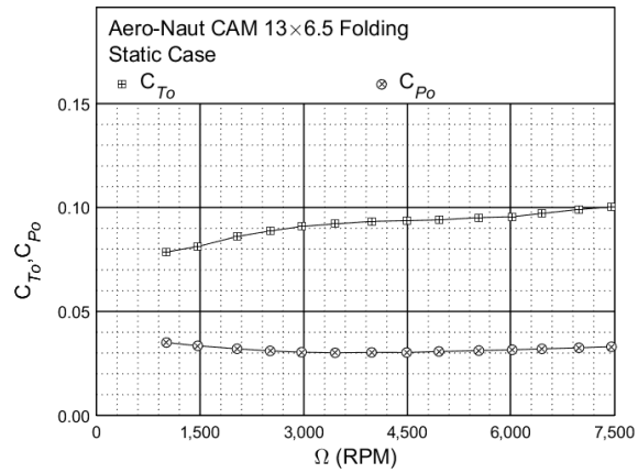
Figure 62: Static performance of the Aero-Naut CAM 13×6.5 folding propeller: thrust and power coefficient.
