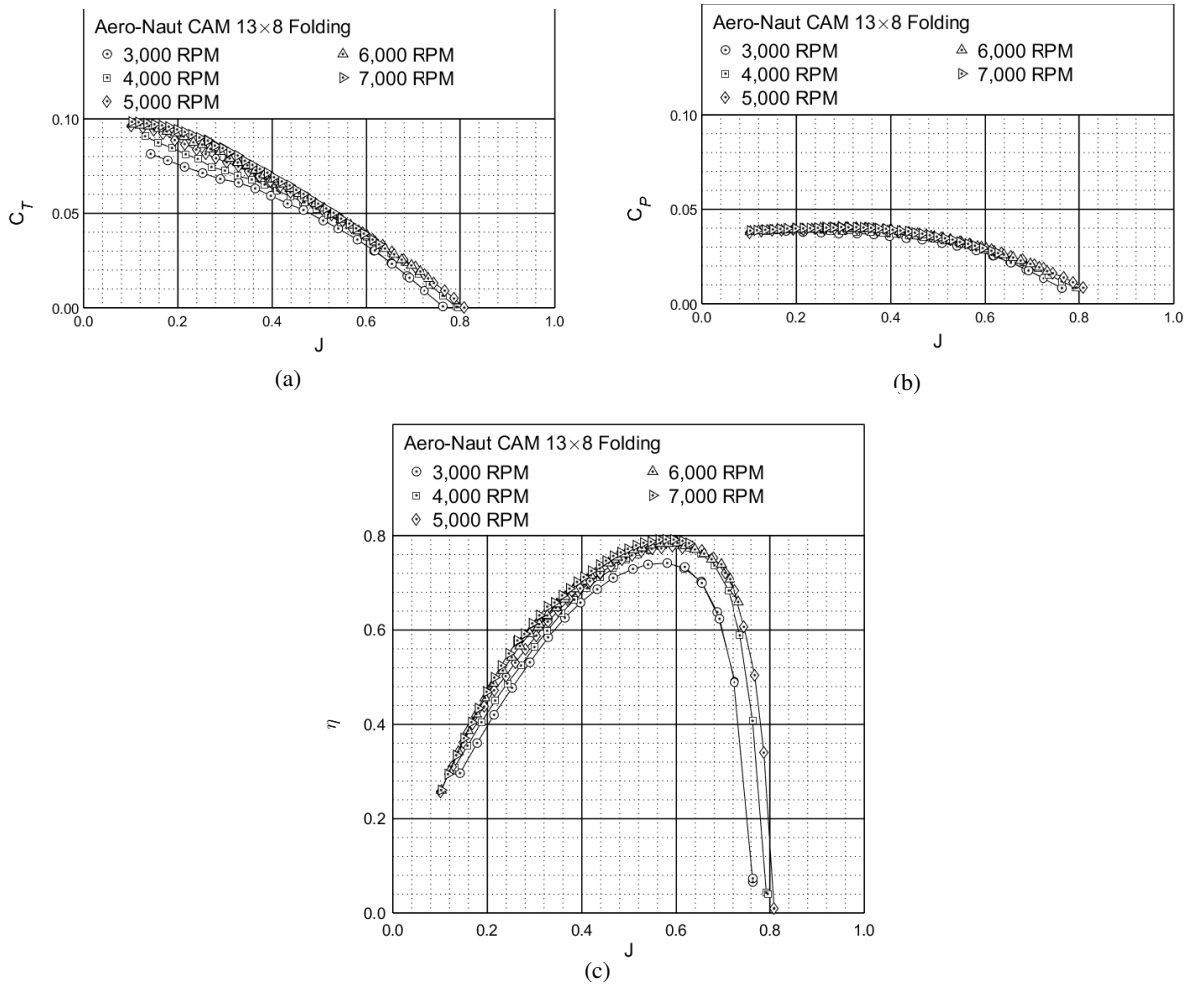
Figure 63: Performance of the Aero-Naut CAM 13×8 folding propeller: (a) thrust coefficient, (b) power coefficient, (c) efficiency.
