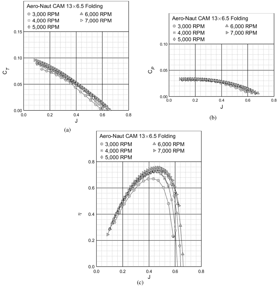
Figure 61: Performance of the Aero-Naut CAM 13×6.5 folding propeller: (a) thrust coefficient, (b) power coefficient, (c) efficiency.
