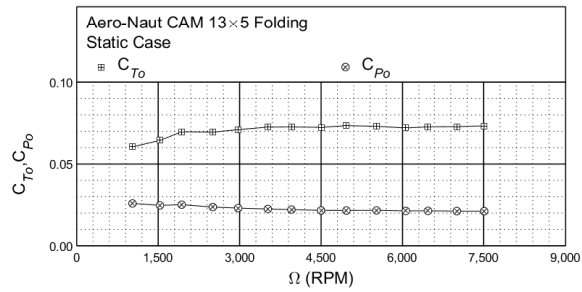
Figure 60: Static performance of the Aero-Naut CAM 13×5 folding propeller: thrust and power coefficient.
