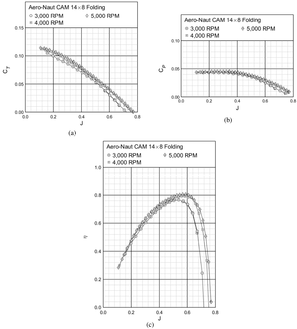
Figure 71: Performance of the Aero-Naut CAM 14x8 folding propeller: (a) thrust coefficient, (b) power coefficient, (c) efficiency.
