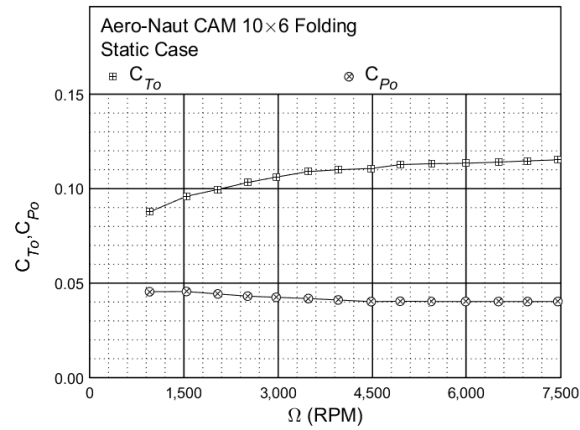
Figure 18: Static performance of the Aero-Naut CAM 10×6 folding propeller: thrust and power coefficient.
