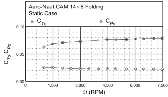
Figure 70: Static performance of the Aero-Naut CAM 14x6 folding propeller: thrust and power coefficient.
